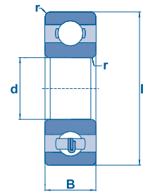
Single row deep groove ball bearing (open)
