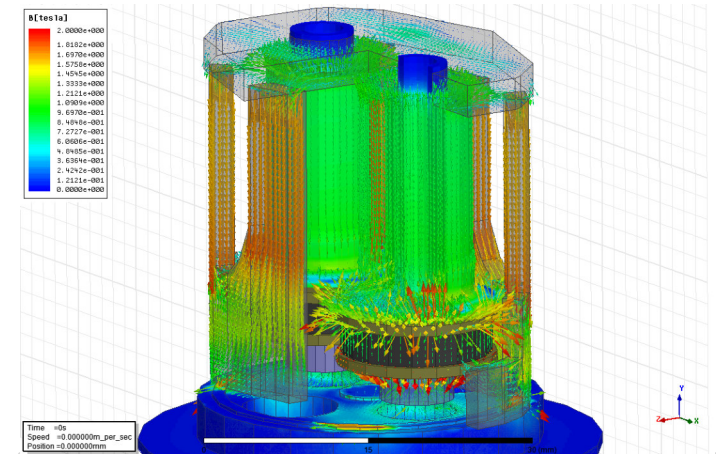
Maxwell / FEMM Magnetic field simulation
