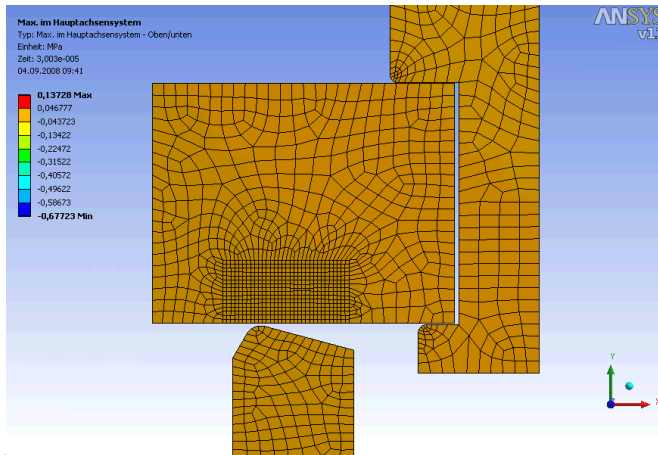
ANSYS MP Linear/non linear structural mechanics
