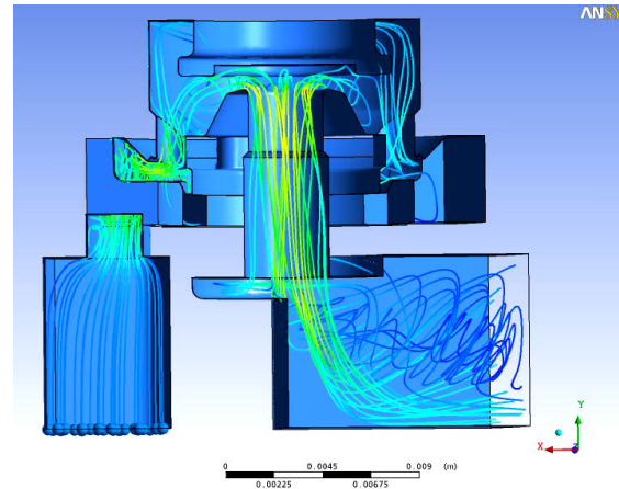
CFX Flow simulation
