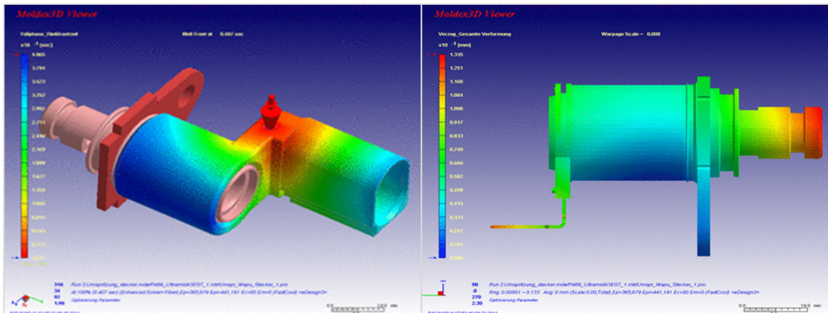
Moldex 3D Plastic simulation e.g. plastic flow with effect of inserts
